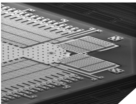
Figure 5. Microelectromechanical structure used for precision motion determination.
